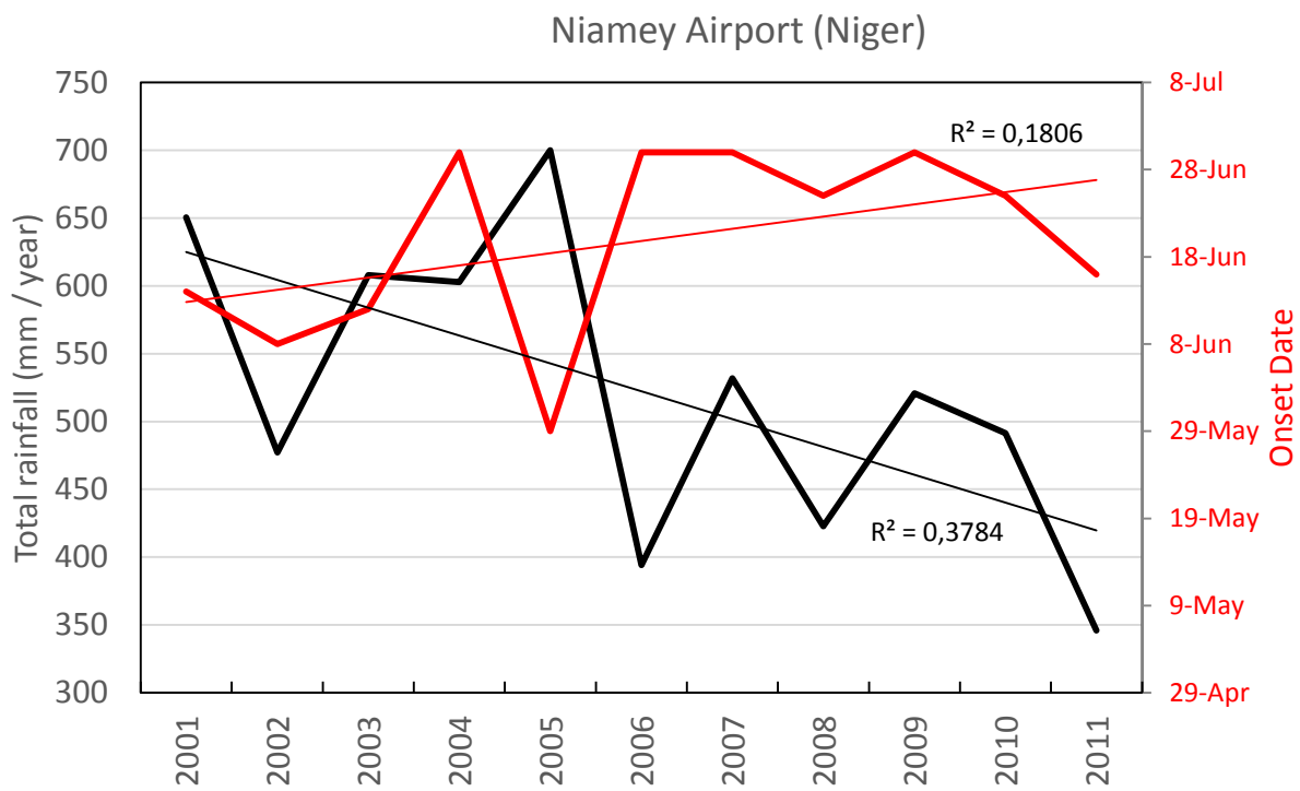
Figure S.2: Time series of total rainfall (black) and onset of the rains (red) measured at the Niamey Airport Meteorological station.
